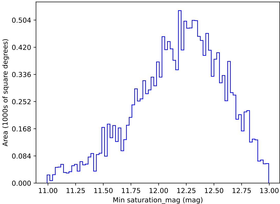
noroll_mjdp270_v3.4_10yrs WFD z band: Min saturation_mag
