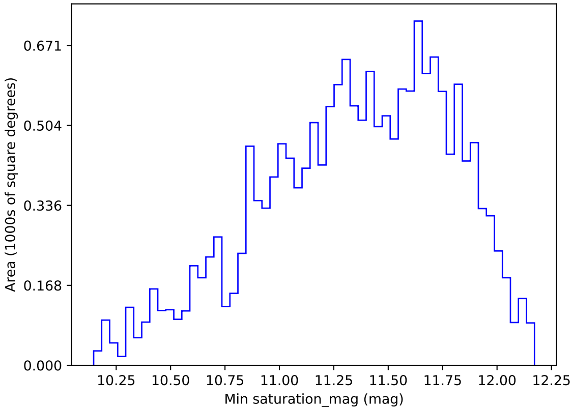
noroll_mjdp270_v3.4_10yrs WFD y band: Min saturation_mag
