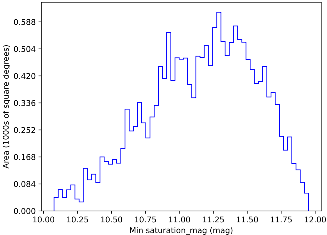
noroll_mjdp270_v3.4_10yrs WFD all bands: Min saturation_mag
