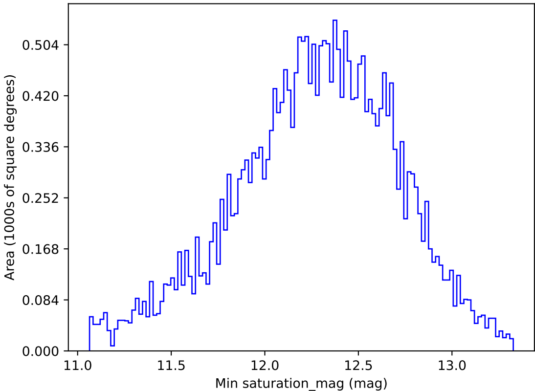
noroll_mjdp270_v3.4_10yrs All sky z band: Min saturation_mag
