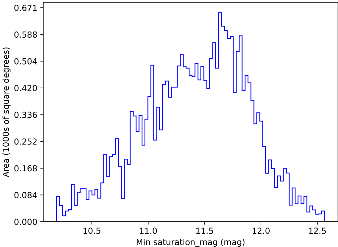
noroll_mjdp270_v3.4_10yrs All sky y band: Min saturation_mag
