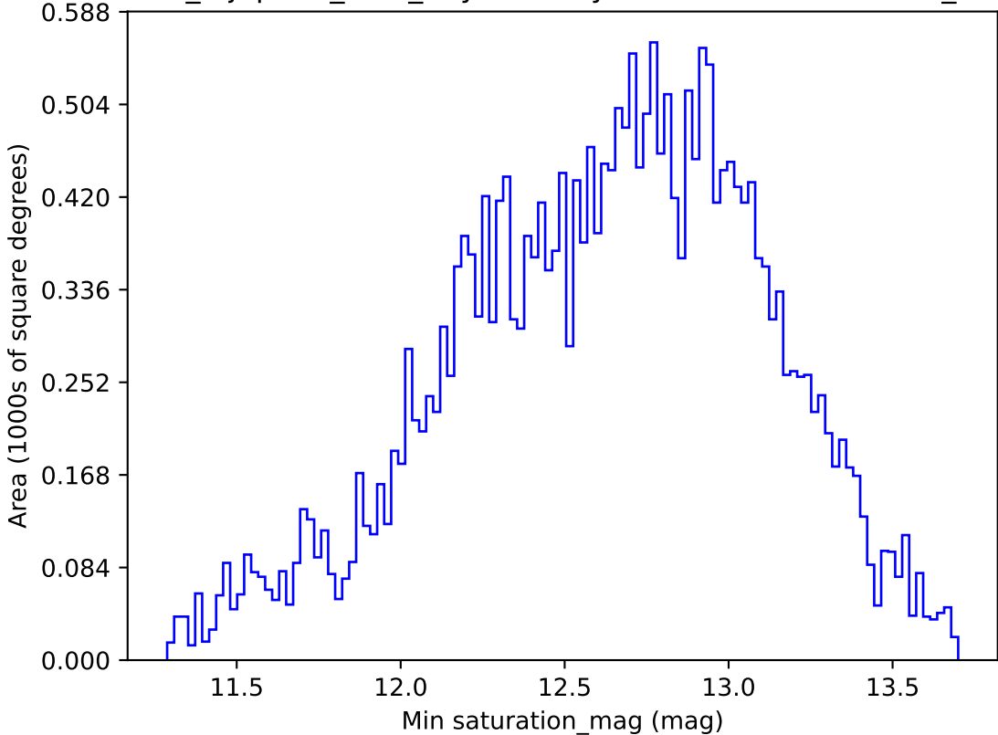
noroll_mjdp270_v3.4_10yrs All sky r band: Min saturation_mag
