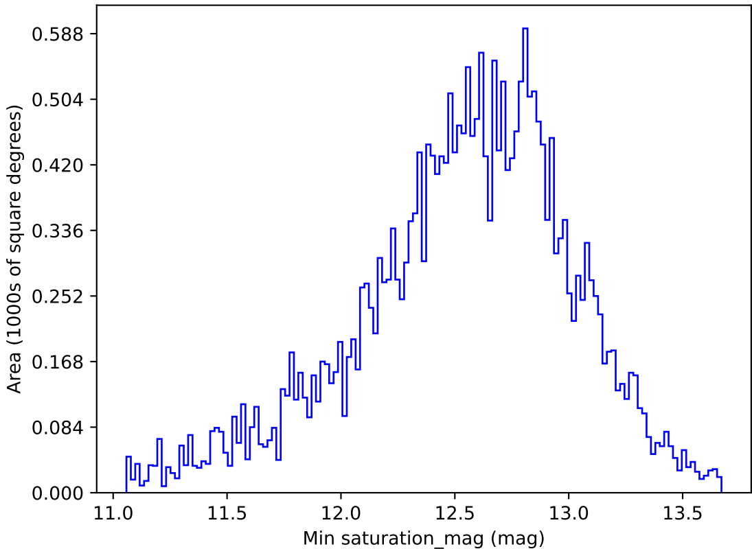
noroll_mjdp270_v3.4_10yrs All sky i band: Min saturation_mag
