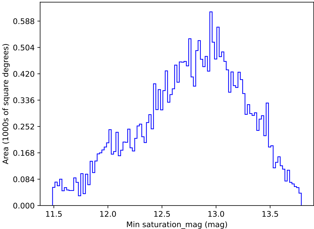
noroll_mjdp270_v3.4_10yrs All sky g band: Min saturation_mag
