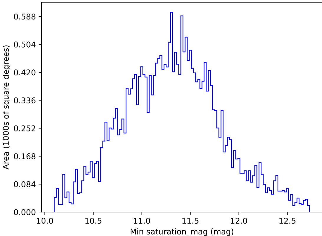
noroll_mjdp270_v3.4_10yrs All sky all bands: Min saturation_mag
