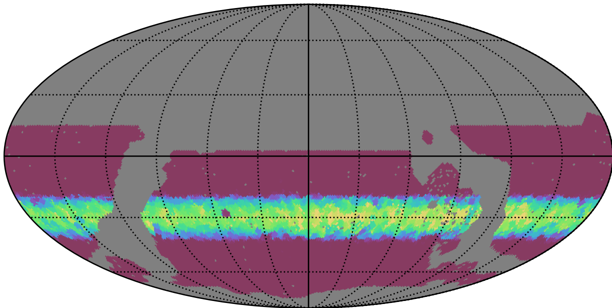
noroll_mjdp270_v3.4_10yrs WFD z band: Min normairmass
