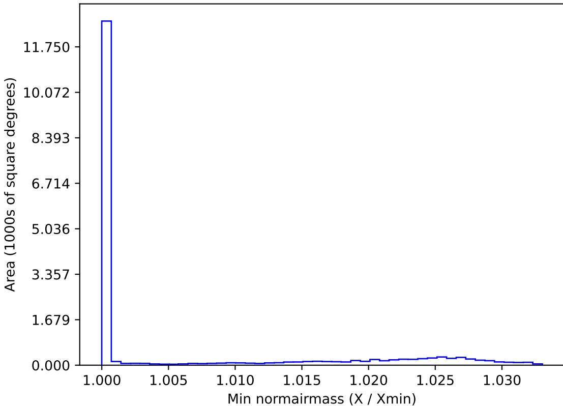
noroll_mjdp270_v3.4_10yrs WFD z band: Min normairmass
