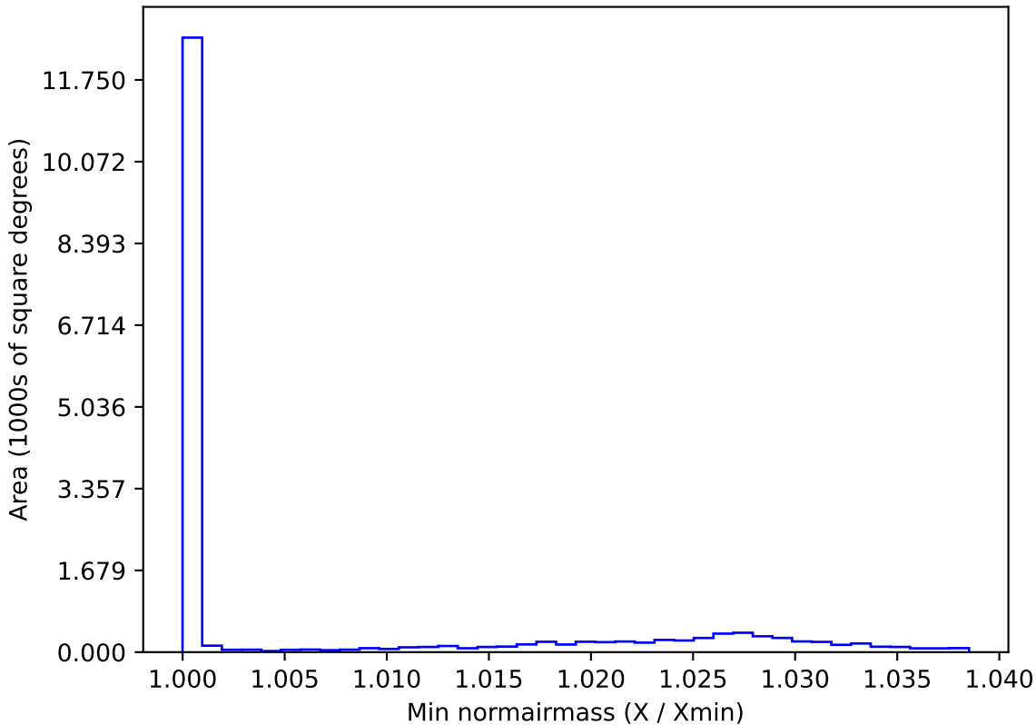
noroll_mjdp270_v3.4_10yrs WFD y band: Min normairmass
