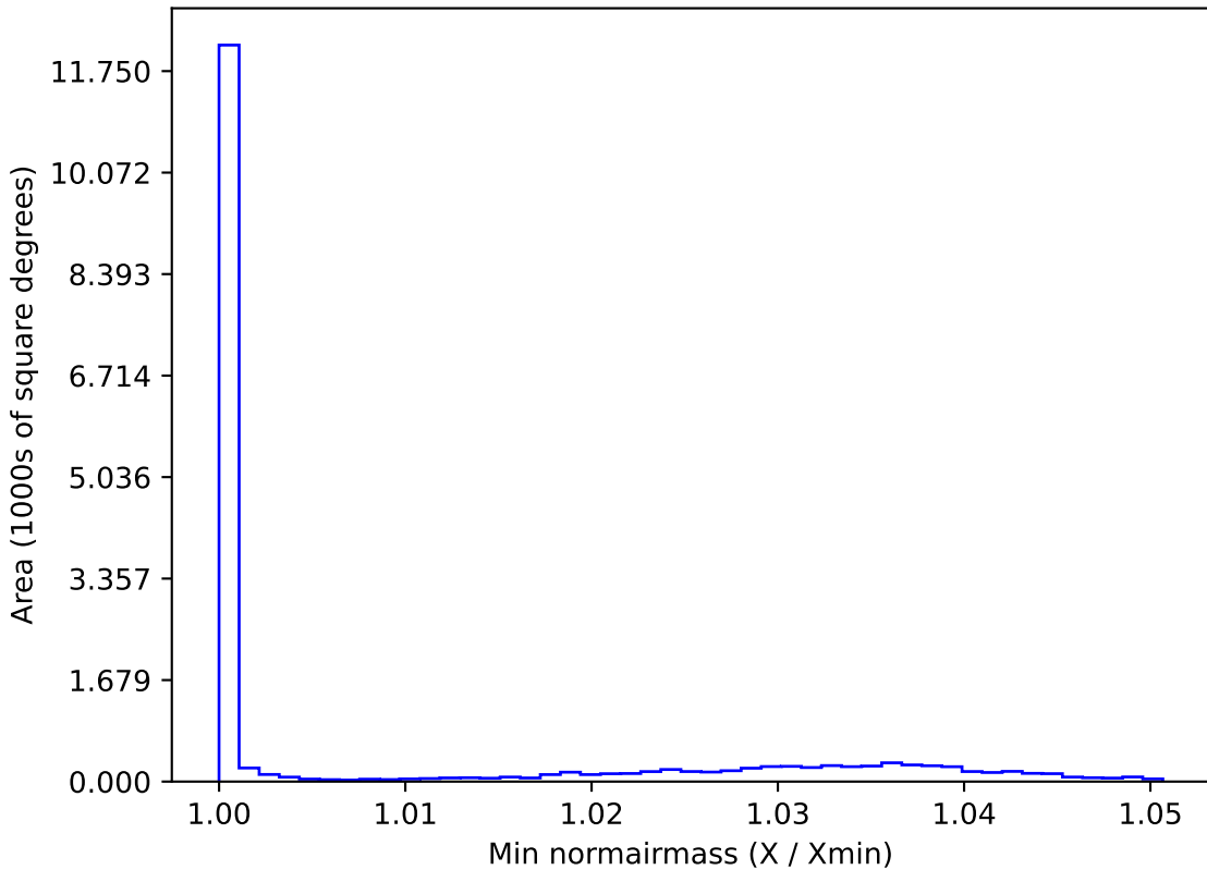
noroll_mjdp270_v3.4_10yrs WFD u band: Min normairmass
