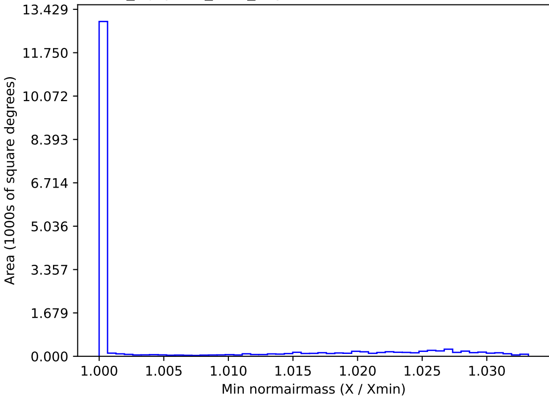
noroll_mjdp270_v3.4_10yrs WFD r band: Min normairmass
