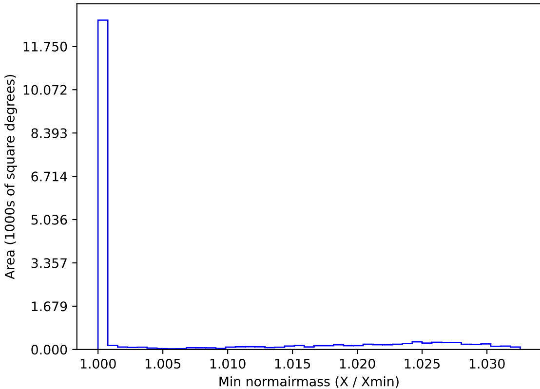
noroll_mjdp270_v3.4_10yrs WFD i band: Min normairmass
