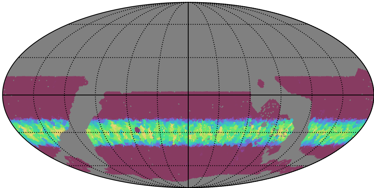
noroll_mjdp270_v3.4_10yrs WFD g band: Min normairmass
