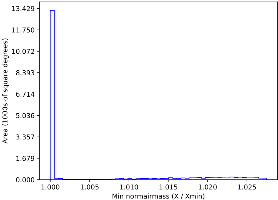
noroll_mjdp270_v3.4_10yrs WFD all bands: Min normairmass
