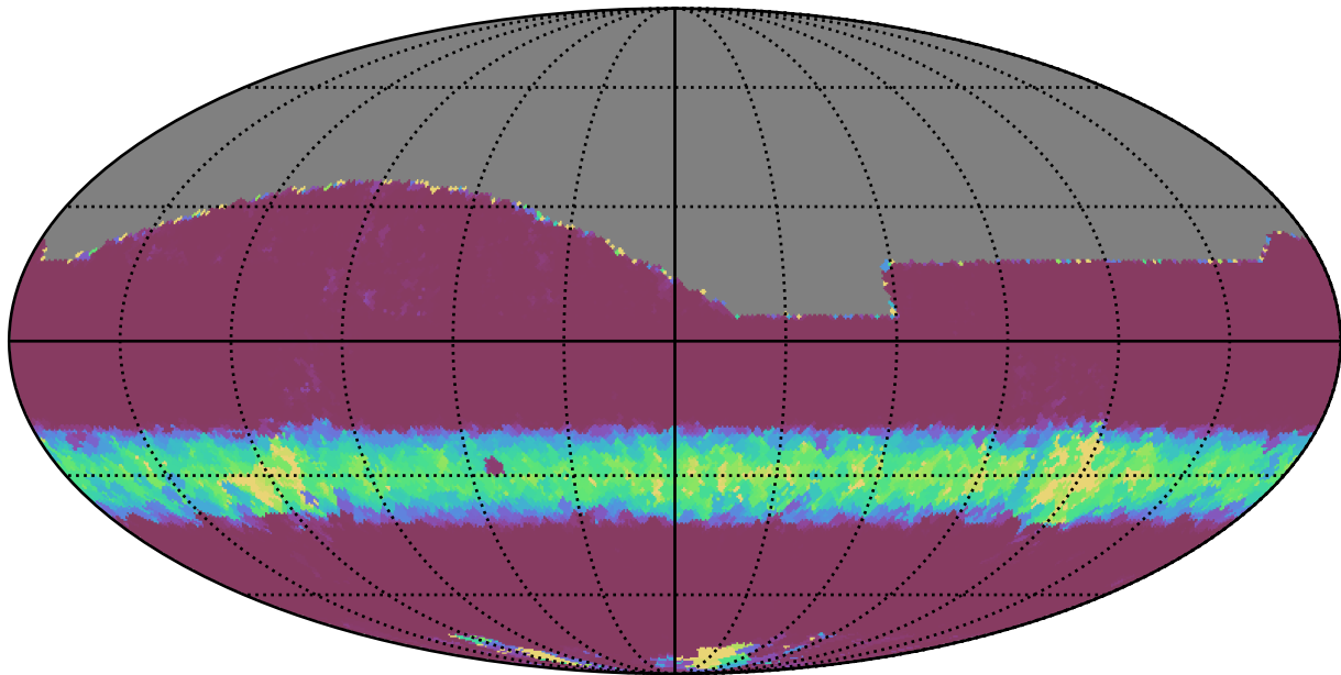
noroll_mjdp270_v3.4_10yrs All sky z band: Min normairmass
