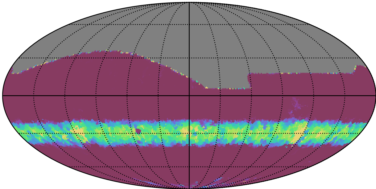
noroll_mjdp270_v3.4_10yrs All sky r band: Min normairmass
