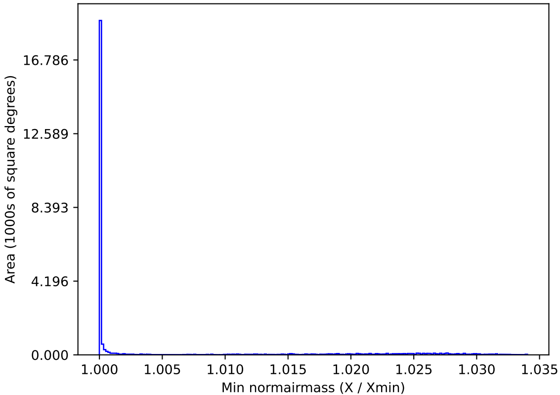
noroll_mjdp270_v3.4_10yrs All sky i band: Min normairmass
