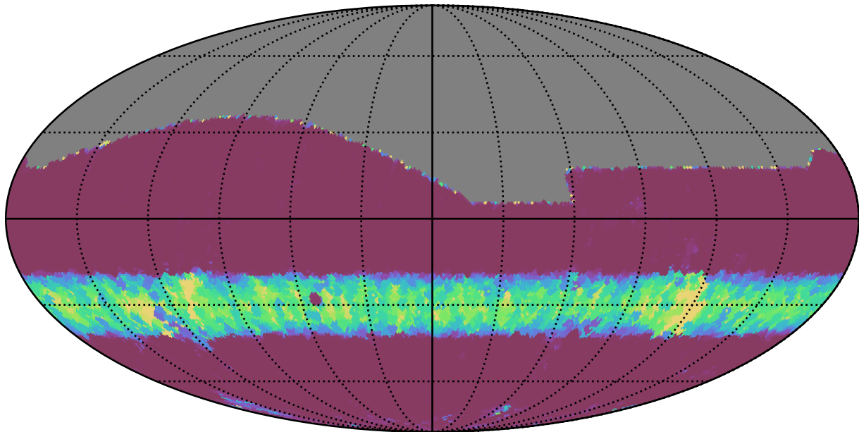
noroll_mjdp270_v3.4_10yrs All sky g band: Min normairmass
