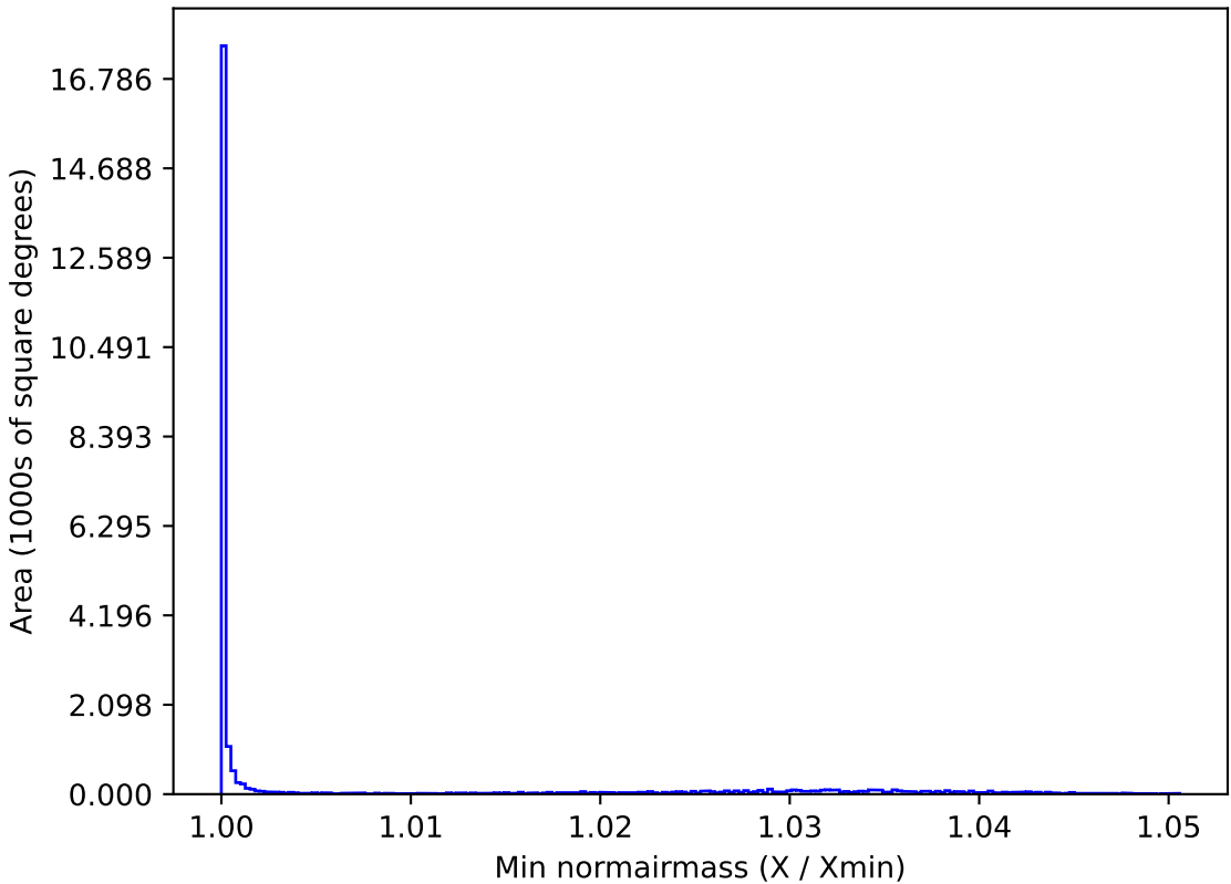
noroll_mjdp270_v3.4_10yrs All sky g band: Min normairmass
