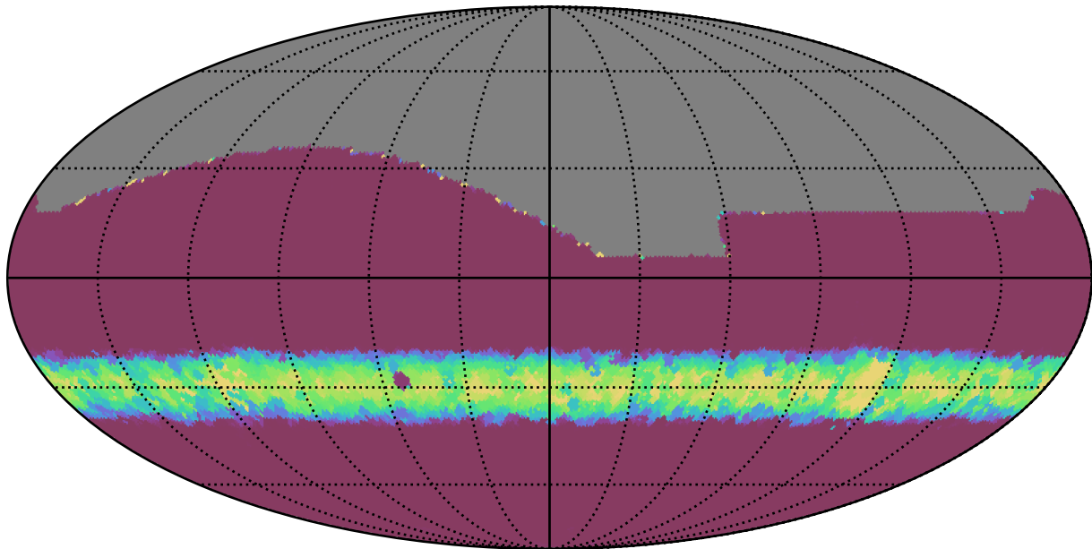
noroll_mjdp270_v3.4_10yrs All sky all bands: Min normairmass
