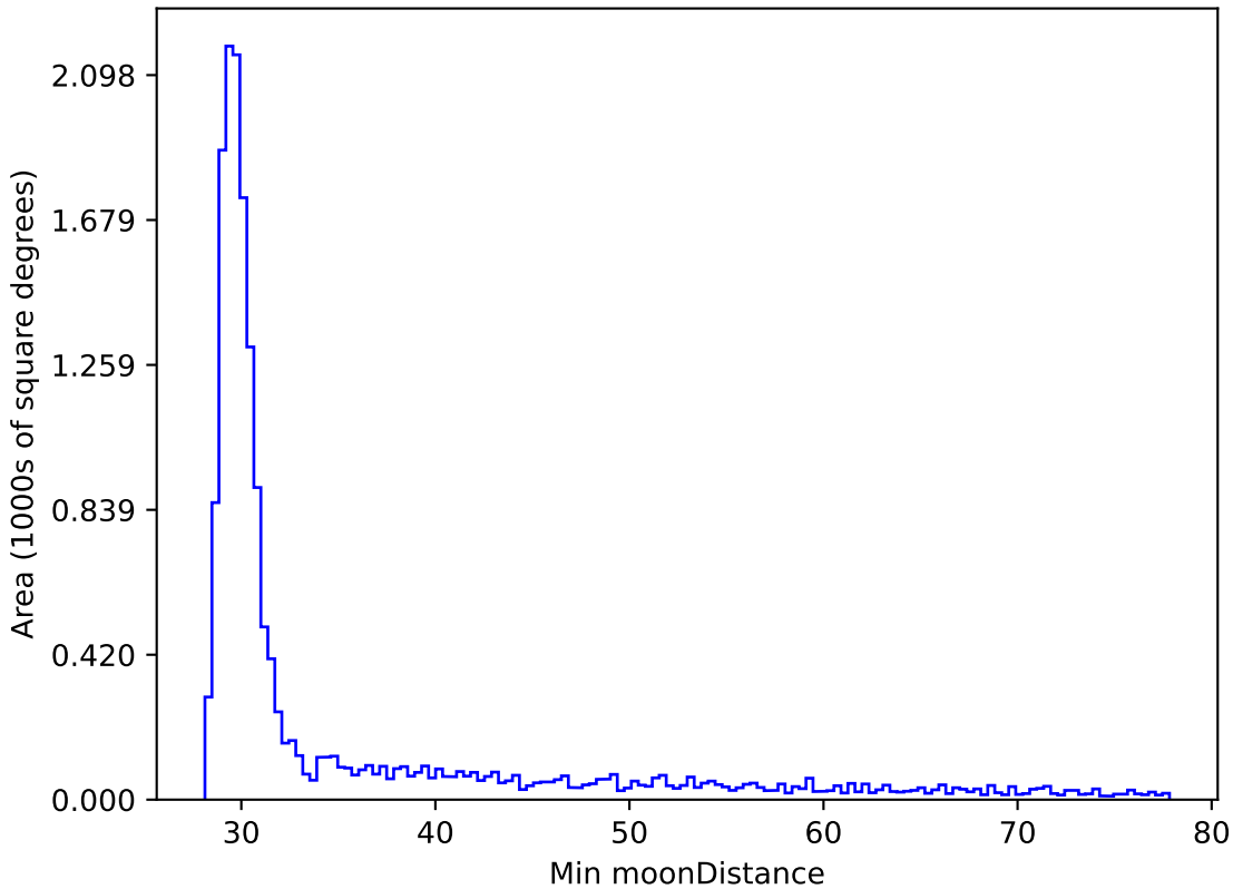
noroll_mjdp270_v3.4_10yrs WFD z band: Min moonDistance
