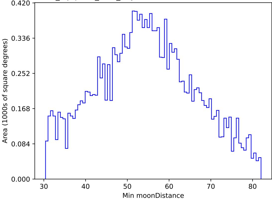
noroll_mjdp270_v3.4_10yrs WFD u band: Min moonDistance
