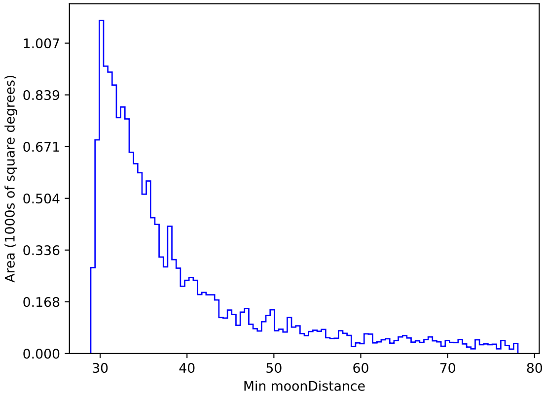
noroll_mjdp270_v3.4_10yrs WFD r band: Min moonDistance
