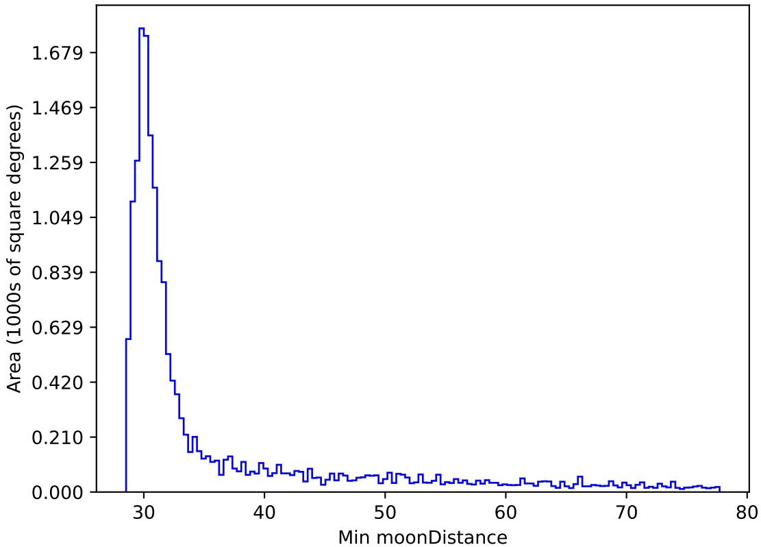
noroll_mjdp270_v3.4_10yrs WFD i band: Min moonDistance
