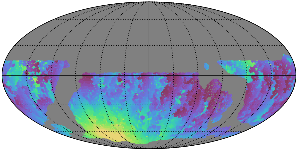
noroll_mjdp270_v3.4_10yrs WFD g band: Min moonDistance
