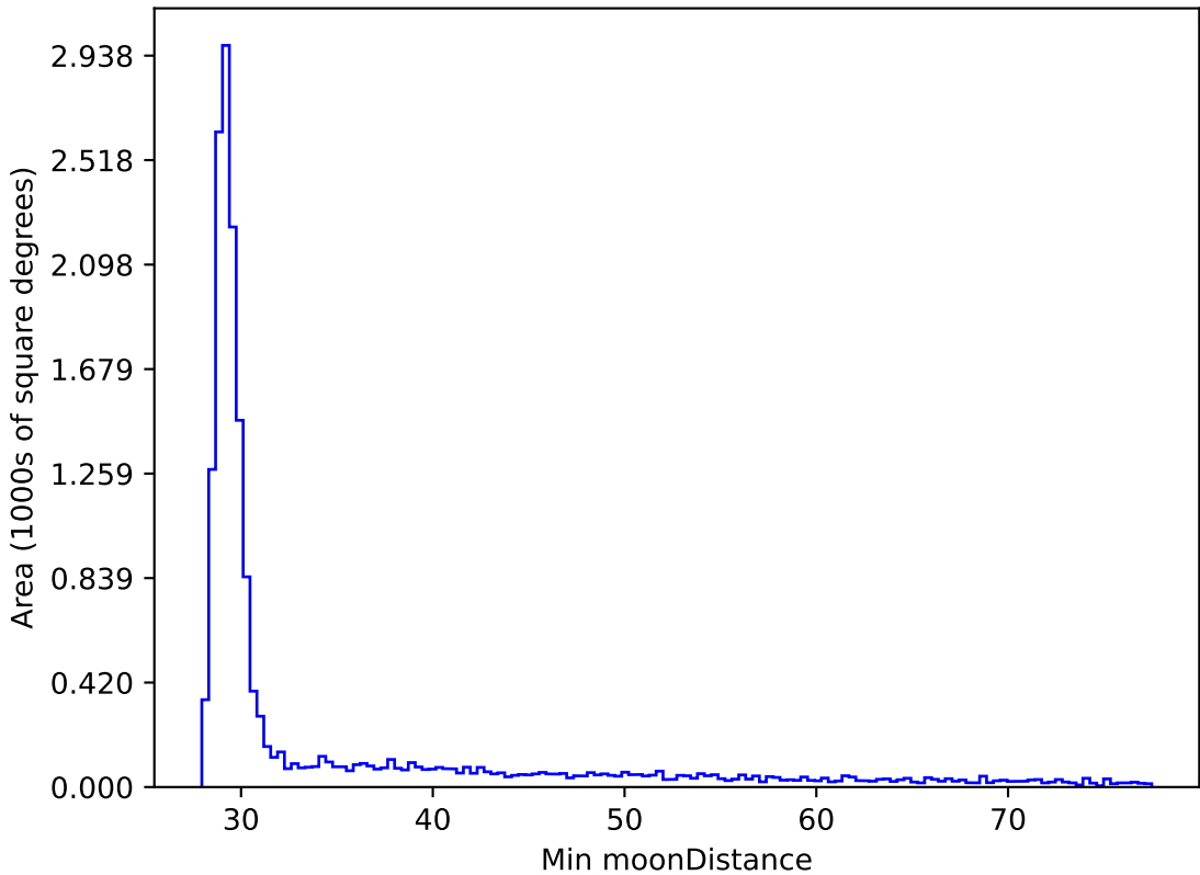
noroll_mjdp270_v3.4_10yrs WFD all bands: Min moonDistance
