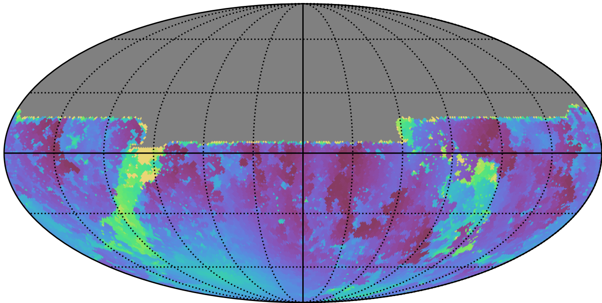
noroll_mjdp270_v3.4_10yrs All sky u band: Min moonDistance
