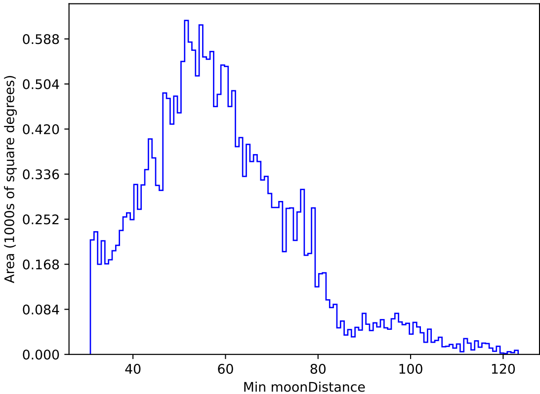
noroll_mjdp270_v3.4_10yrs All sky u band: Min moonDistance
