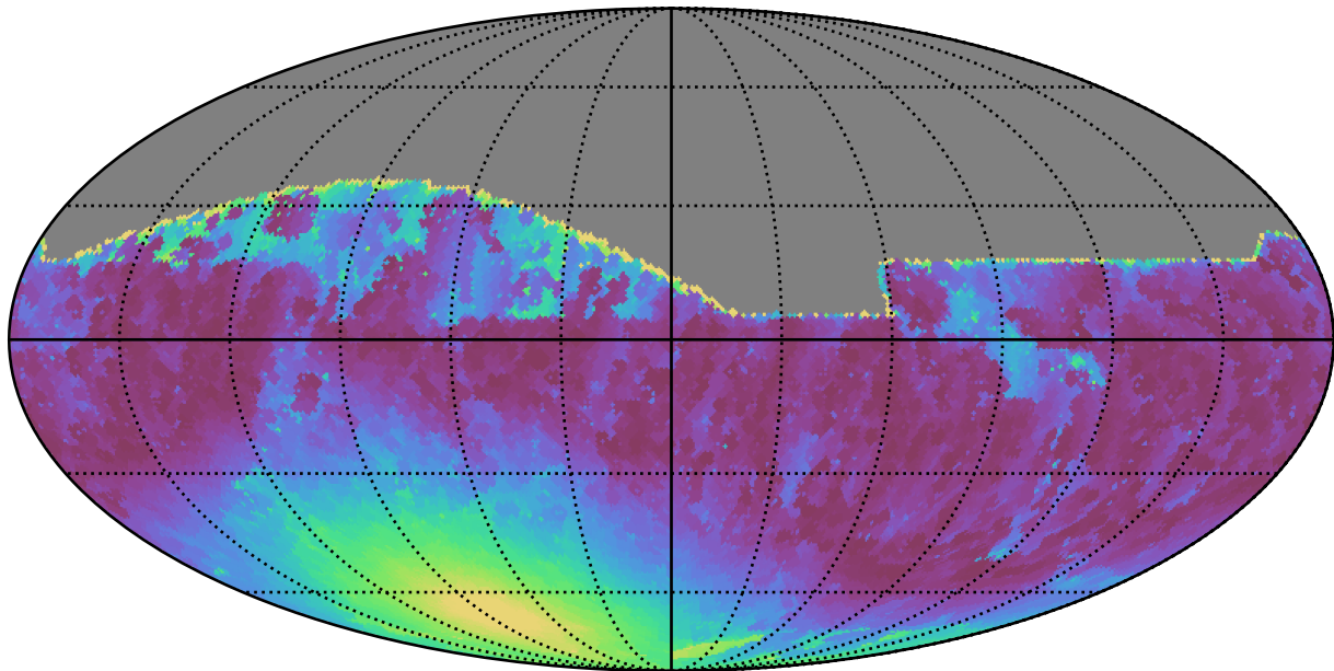
noroll_mjdp270_v3.4_10yrs All sky r band: Min moonDistance
