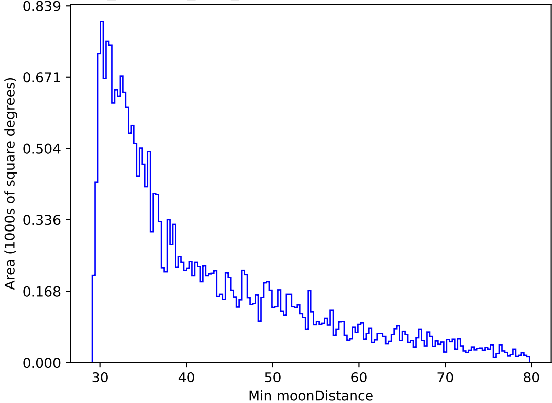
noroll_mjdp270_v3.4_10yrs All sky r band: Min moonDistance
