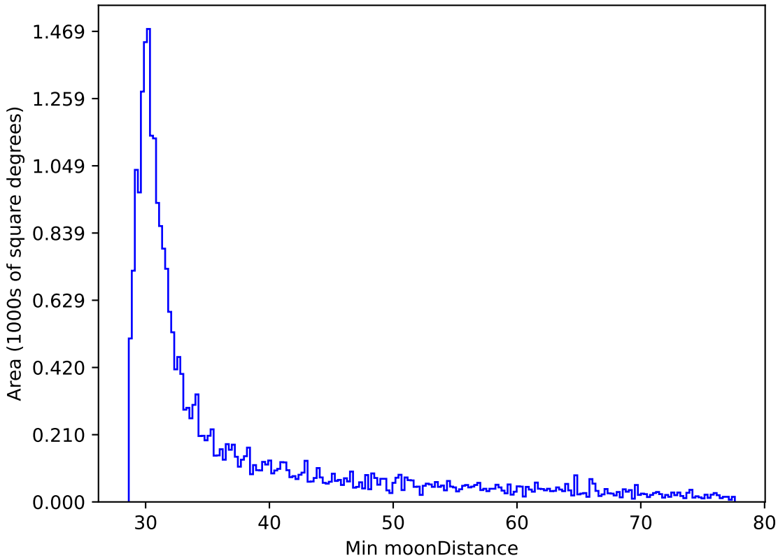
noroll_mjdp270_v3.4_10yrs All sky i band: Min moonDistance
