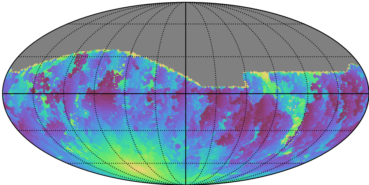
noroll_mjdp270_v3.4_10yrs All sky g band: Min moonDistance
