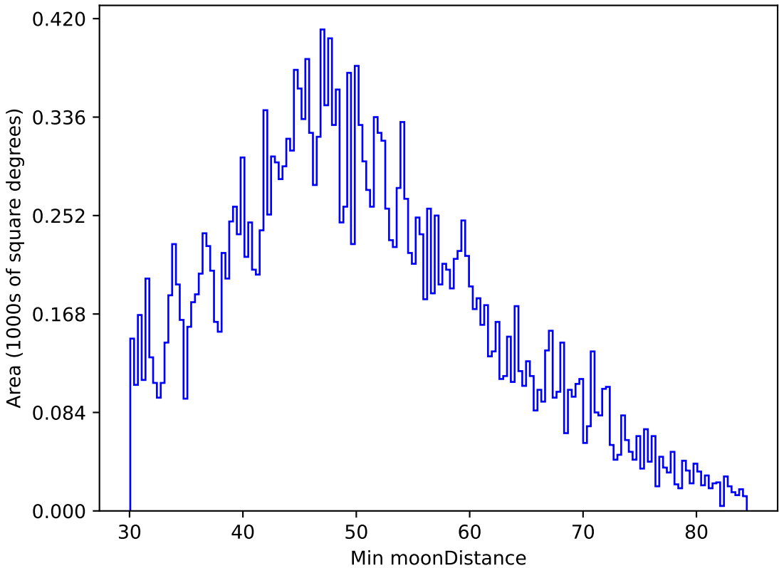
noroll_mjdp270_v3.4_10yrs All sky g band: Min moonDistance
