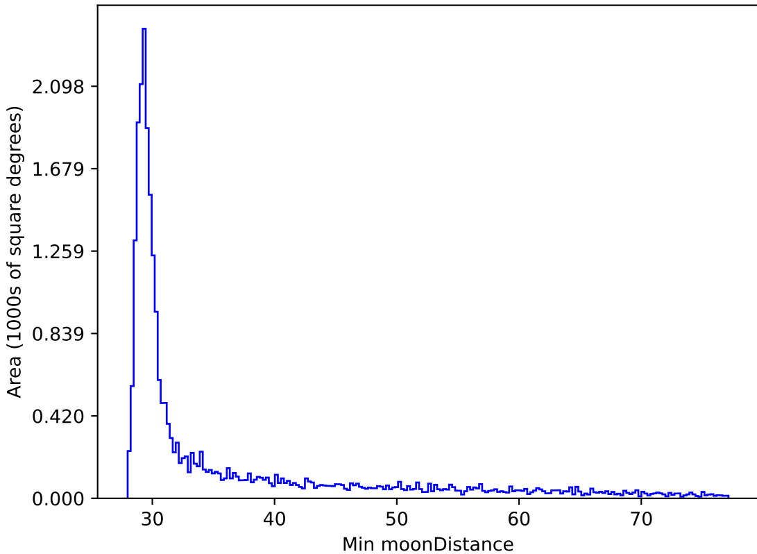
noroll_mjdp270_v3.4_10yrs All sky all bands: Min moonDistance
