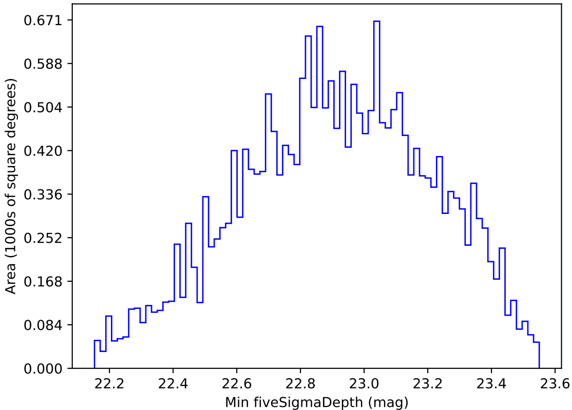
noroll_mjdp270_v3.4_10yrs Yr 1 u band: Min fiveSigmaDepth
