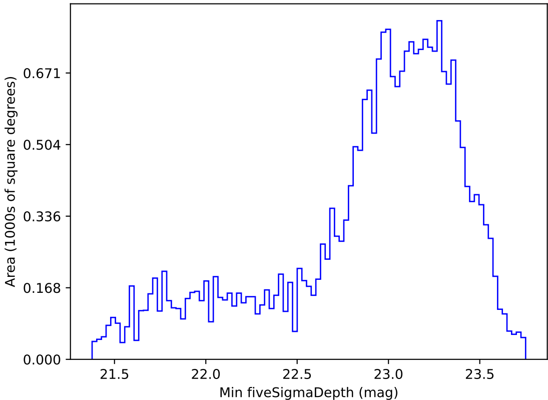
noroll_mjdp270_v3.4_10yrs Yr 1 i band: Min fiveSigmaDepth
