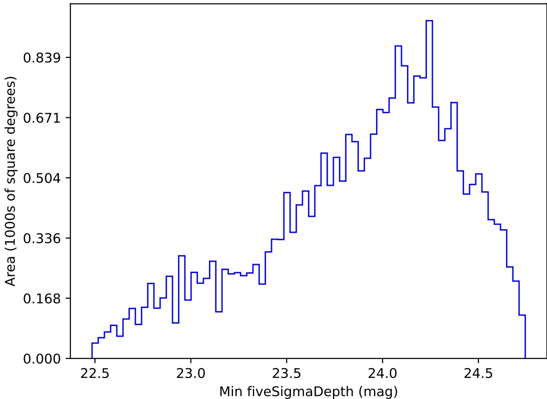
noroll_mjdp270_v3.4_10yrs Yr 1 g band: Min fiveSigmaDepth
