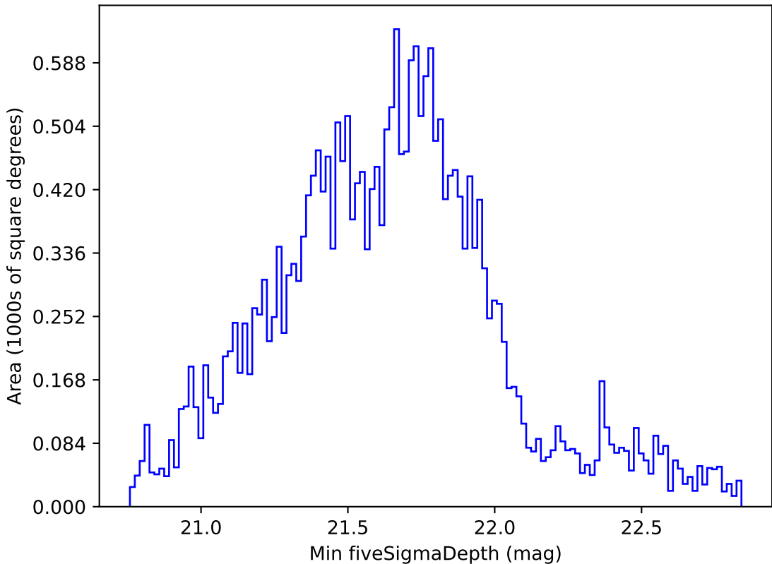
noroll_mjdp270_v3.4_10yrs Yr 1 all bands: Min fiveSigmaDepth
