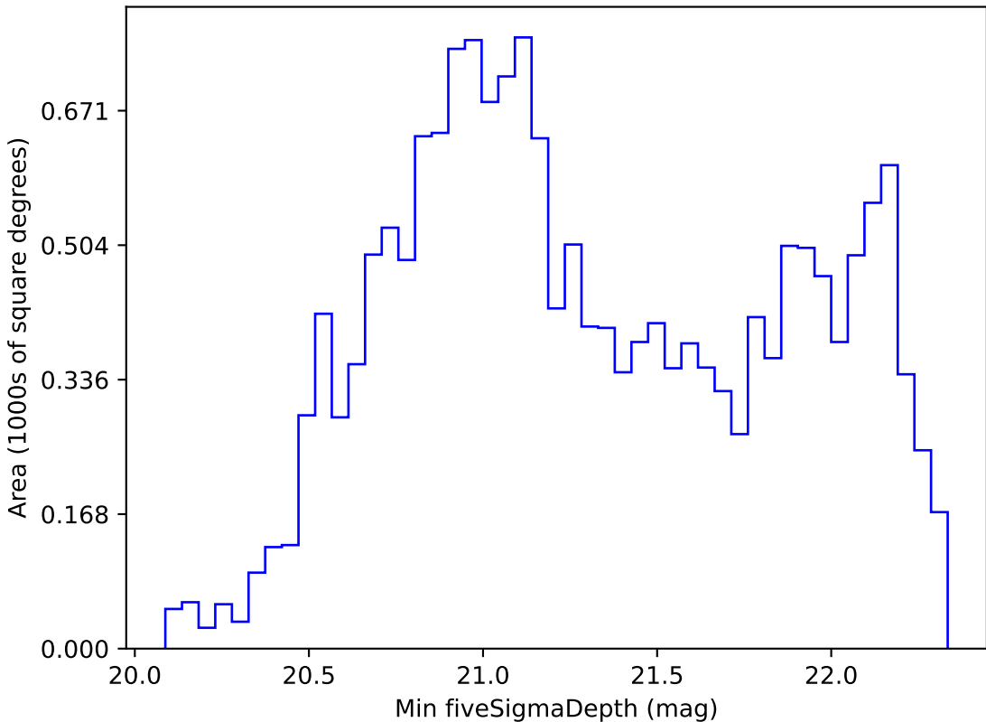
noroll_mjdp270_v3.4_10yrs WFD z band: Min fiveSigmaDepth
