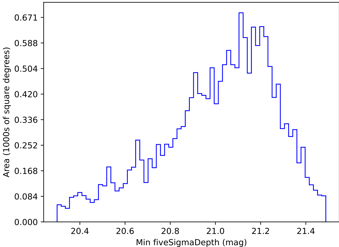
noroll_mjdp270_v3.4_10yrs WFD y band: Min fiveSigmaDepth
