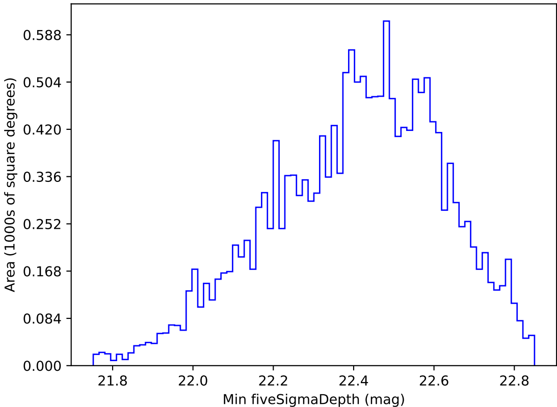
noroll_mjdp270_v3.4_10yrs WFD u band: Min fiveSigmaDepth
