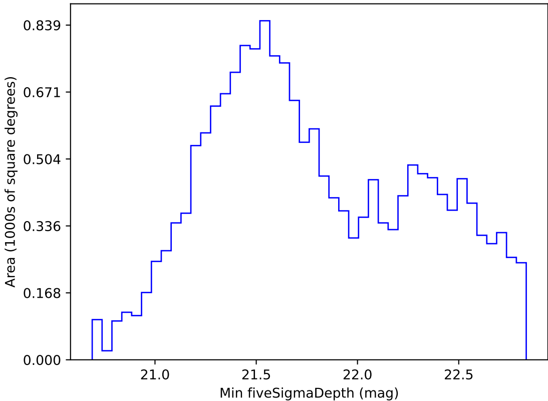
noroll_mjdp270_v3.4_10yrs WFD i band: Min fiveSigmaDepth
