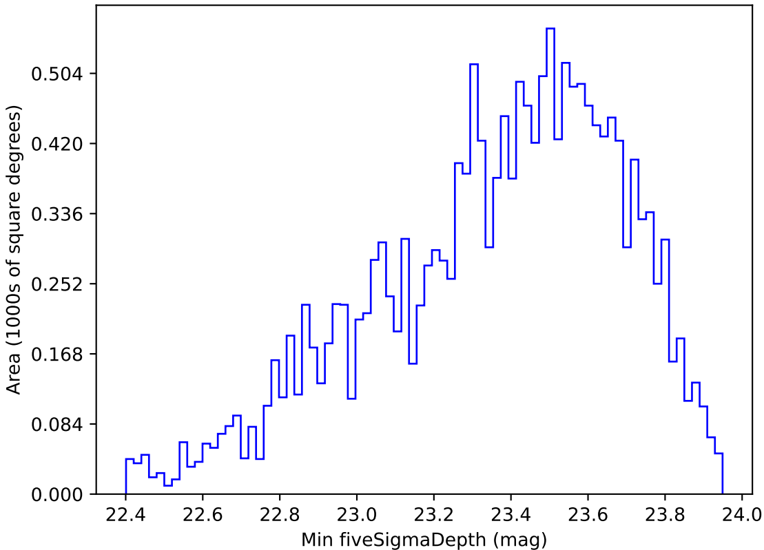
noroll_mjdp270_v3.4_10yrs WFD g band: Min fiveSigmaDepth
