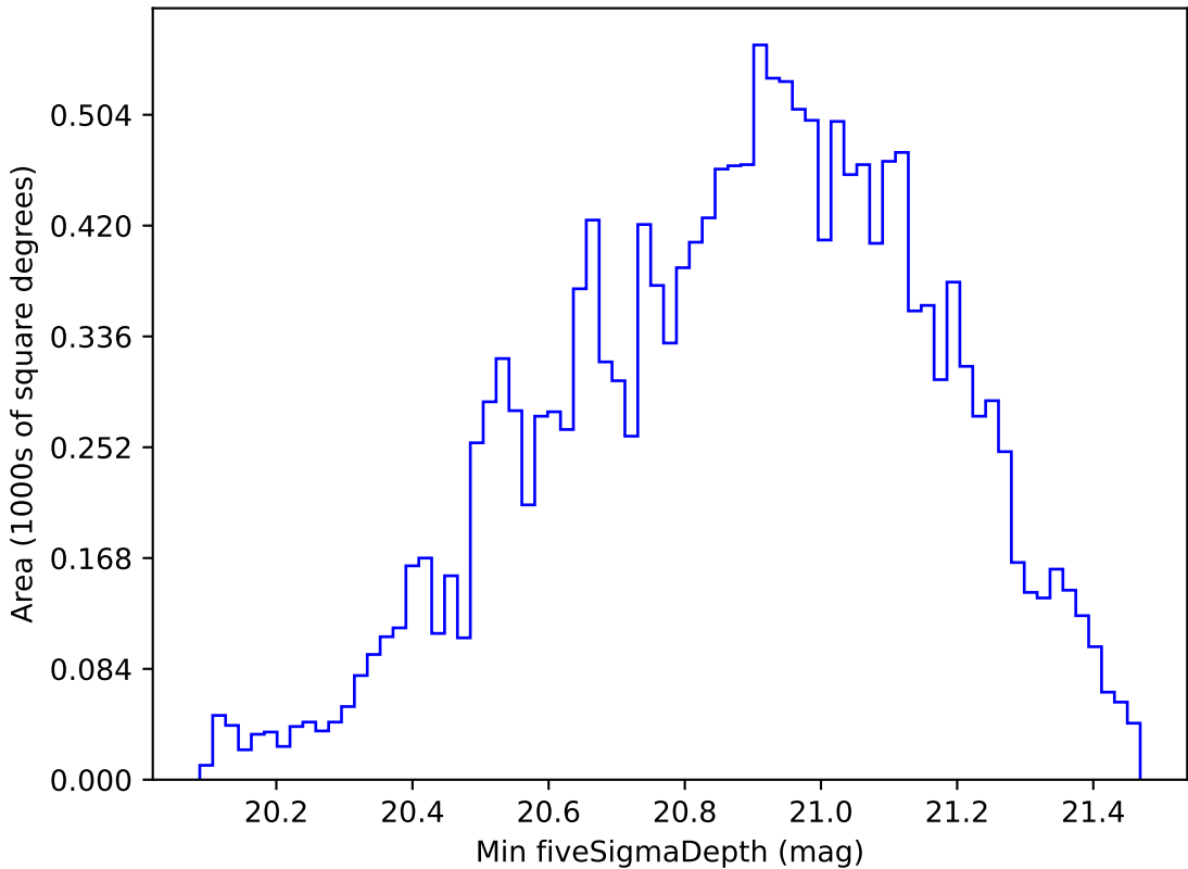
noroll_mjdp270_v3.4_10yrs WFD all bands: Min fiveSigmaDepth
