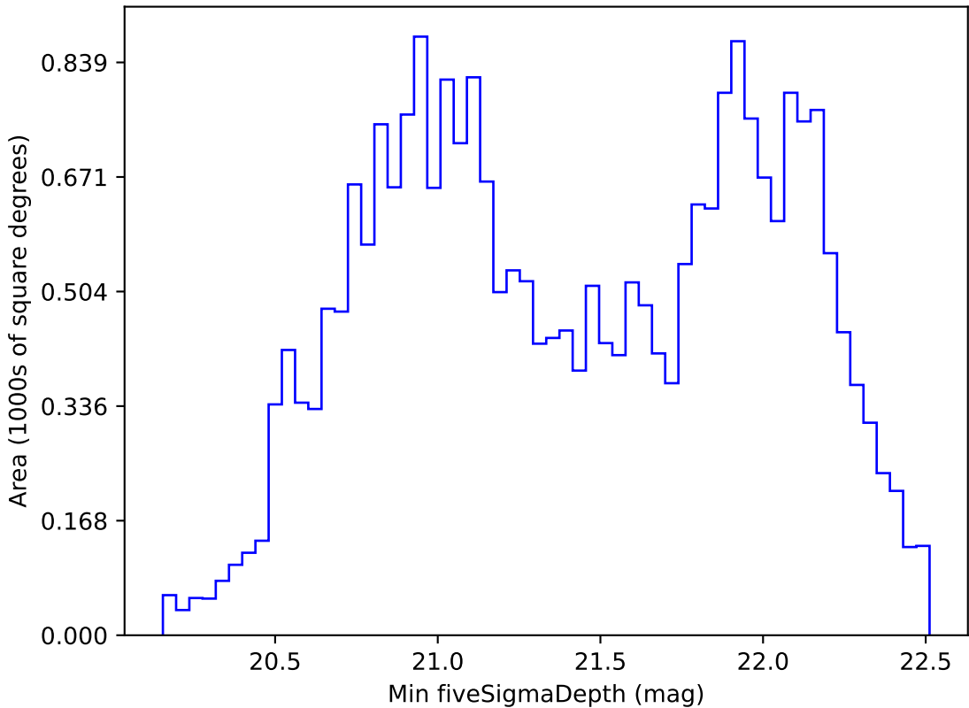
noroll_mjdp270_v3.4_10yrs All sky z band: Min fiveSigmaDepth
