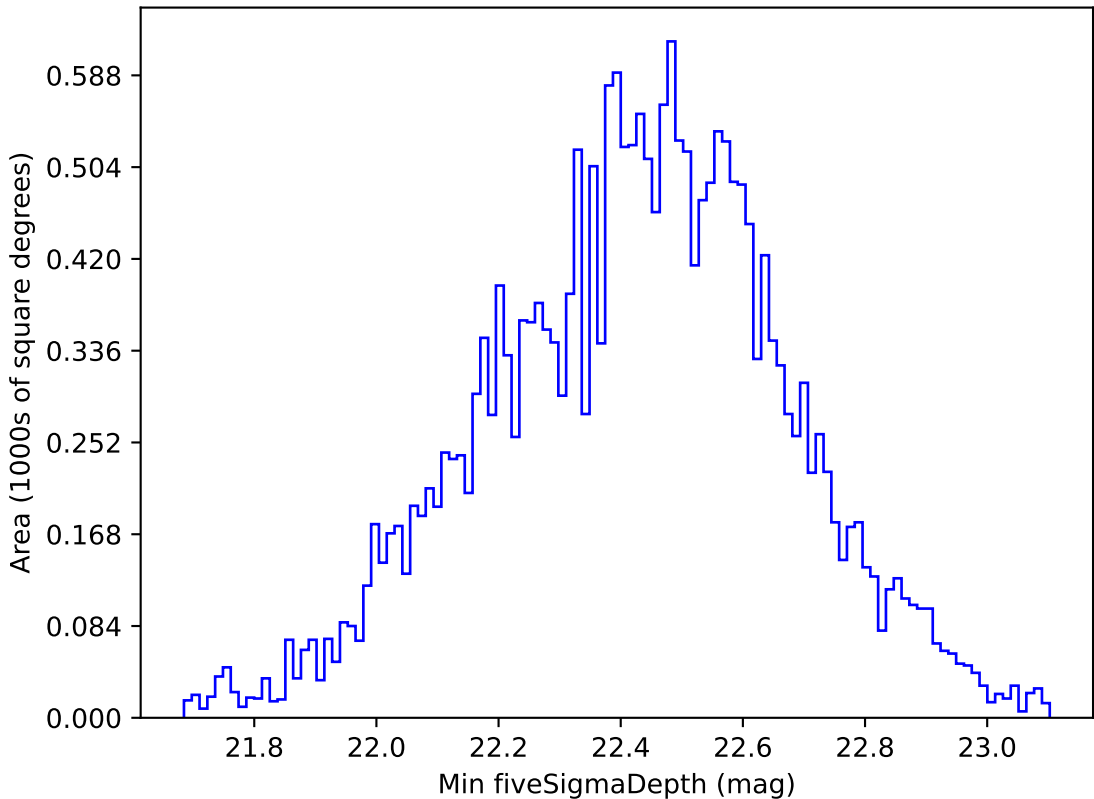
noroll_mjdp270_v3.4_10yrs All sky u band: Min fiveSigmaDepth
