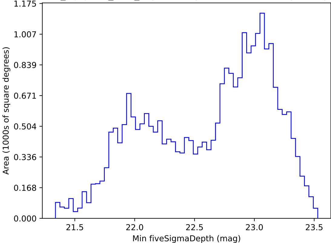
noroll_mjdp270_v3.4_10yrs All sky r band: Min fiveSigmaDepth
